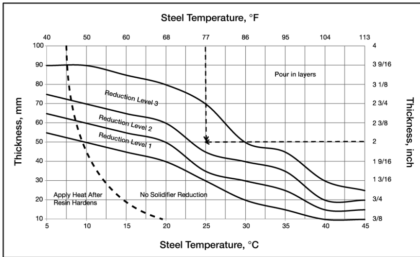
GRAPH 2 - BELZONA 7111 BETWEEN STEEL AND CONCRETE
