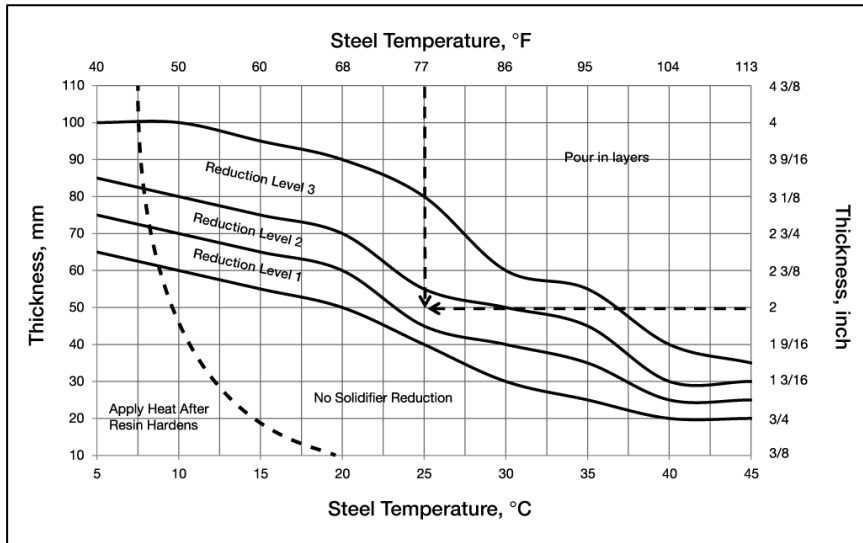
GRAPH 1 - BELZONA 7111 BETWEEN STEEL AND STEEL
